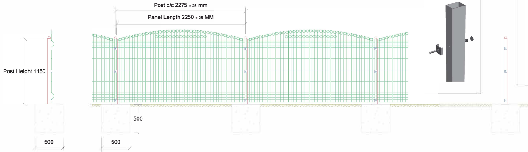
Clips And Plastic Caps Detail
